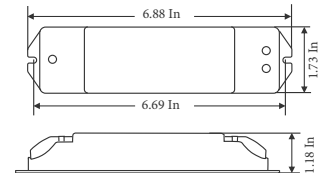
Receiver
