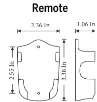
Remote Holder
